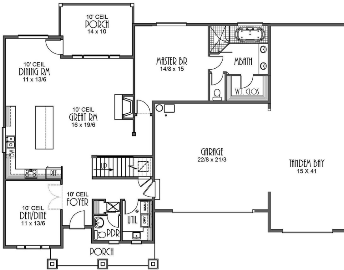
MAIN FLOOR PLAN 1580 SQUARE FEET
