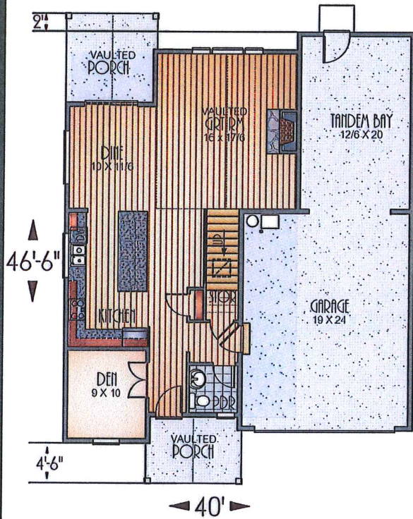
MAIN FLOOR PLAN 920 SQUARE FEET 1792 SQUARE FEET TOTAL
