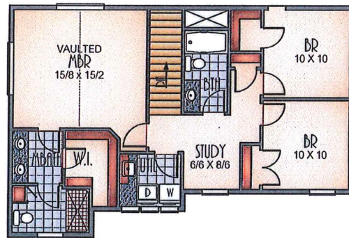
UPPER FLOOR PLAN 872 SQUARE FEET
