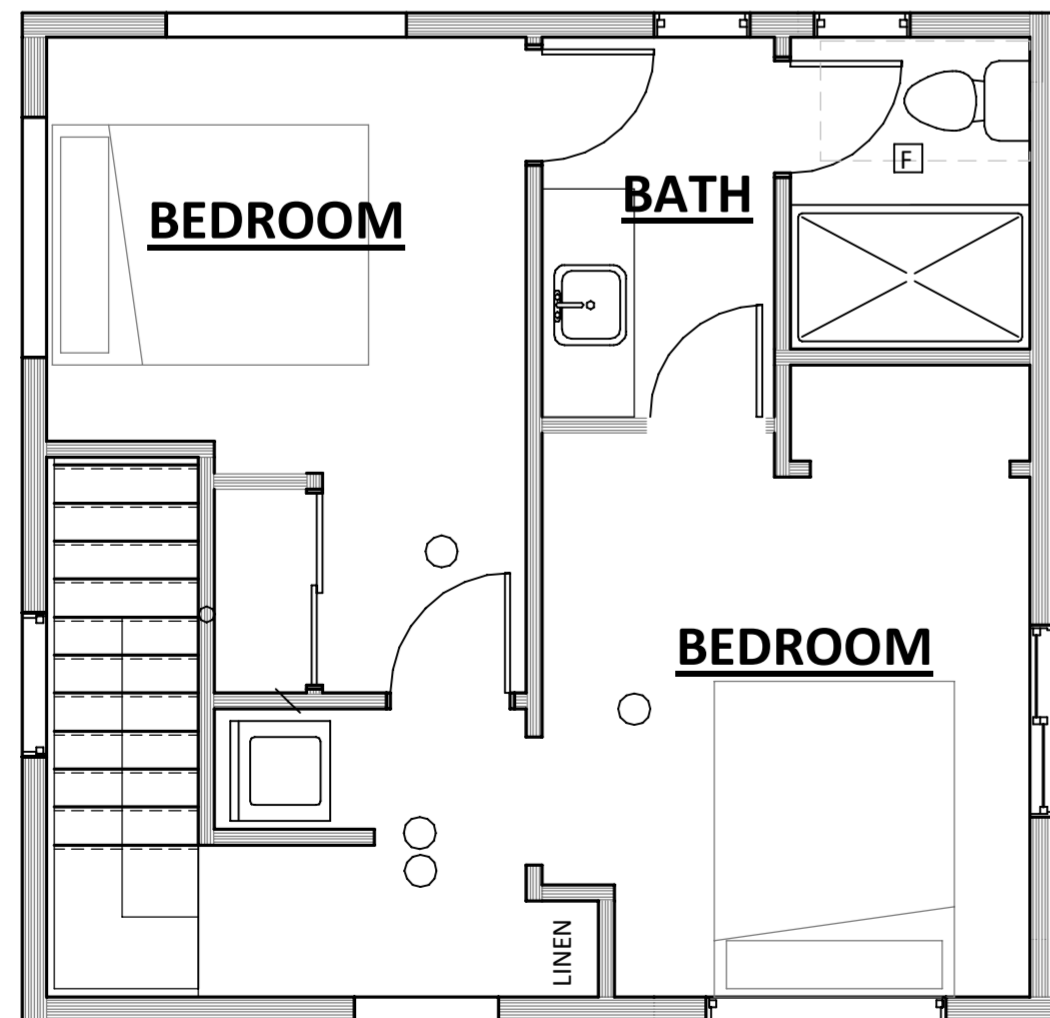
SECOND FLOOR PLAN - 410 S.F.
