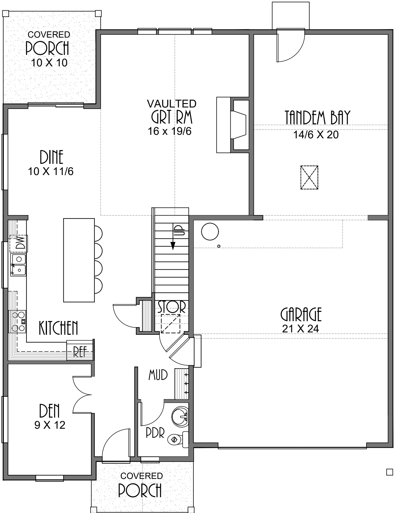
MAIN FLOOR PLAN 1015 SQUARE FEET
