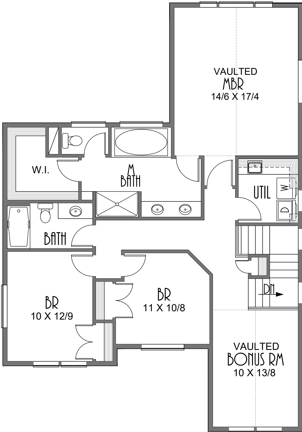
UPPER FLOOR PLAN 1211 SQUARE FEET
