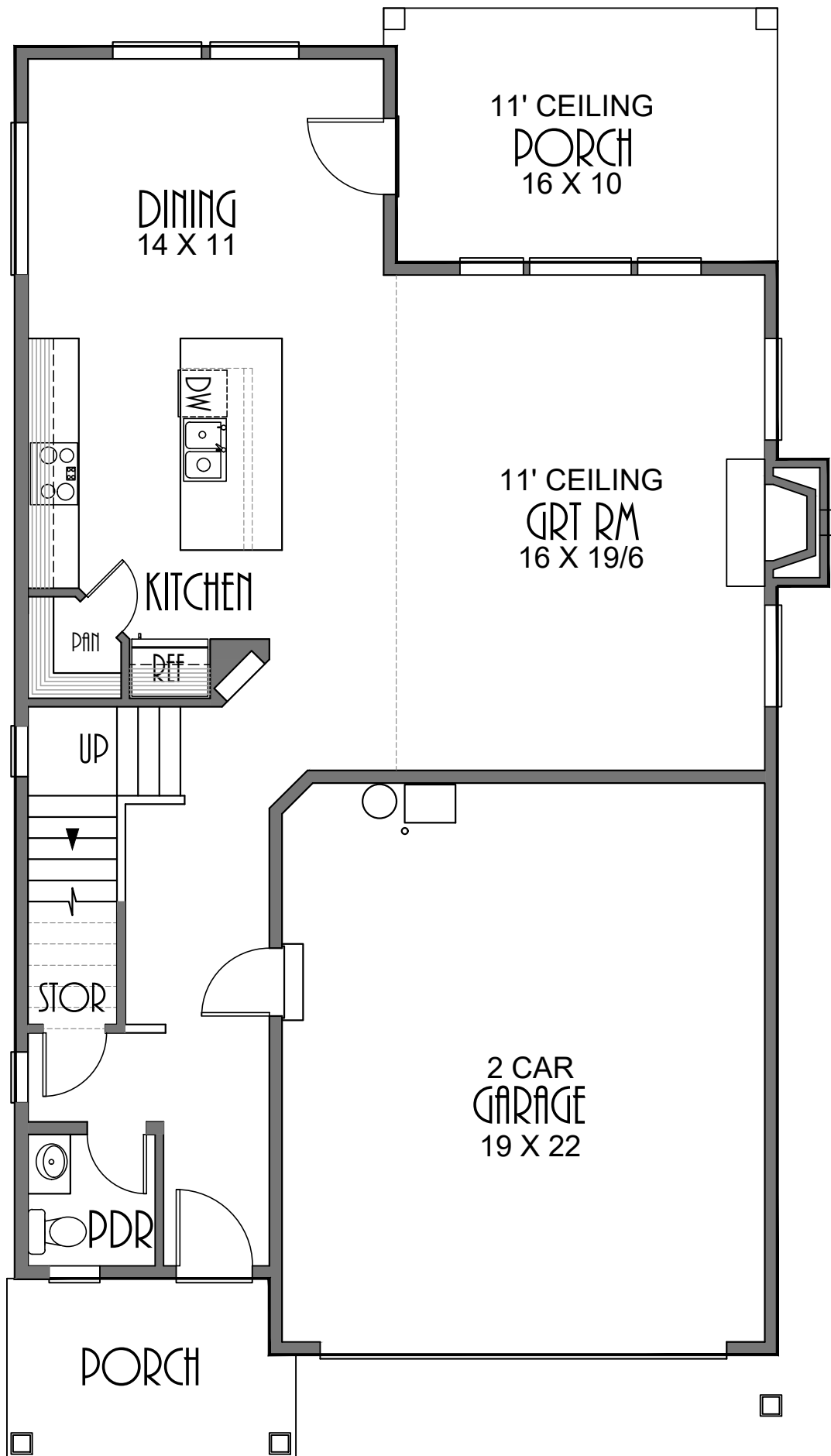
MAIN FLOOR PLAN 947 SQUARE FEET
