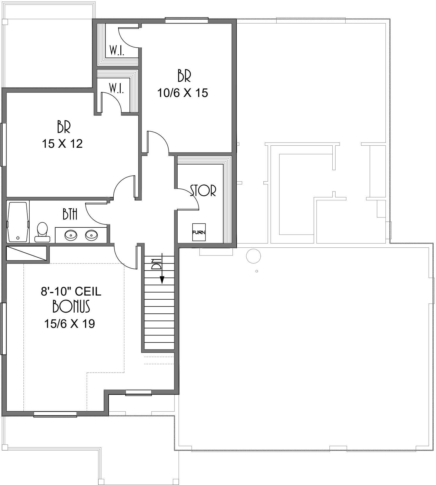
UPPER FLOOR PLAN 964 SQUARE FEET
