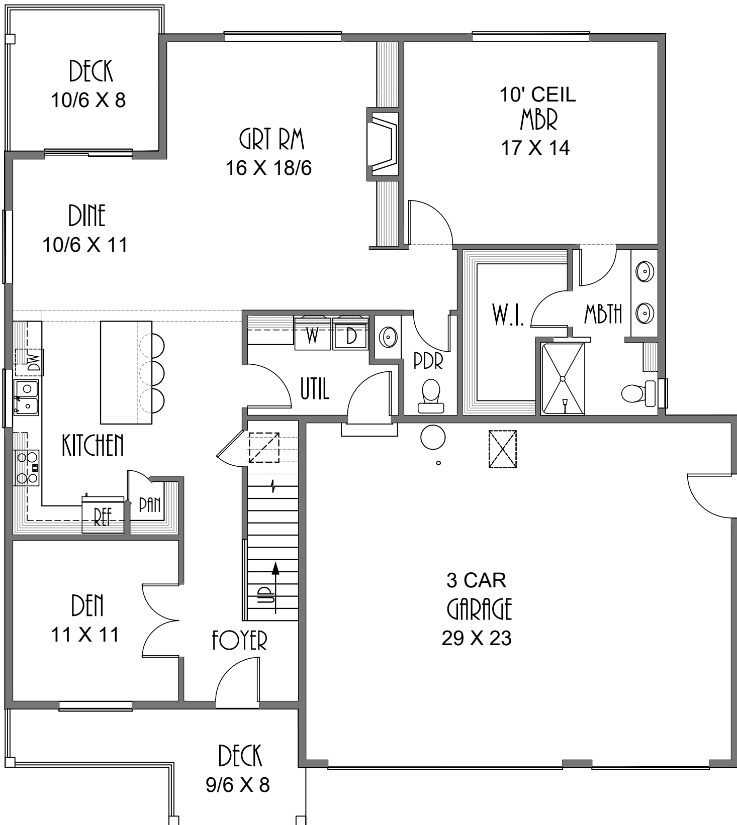
MAIN FLOOR PLAN 1485 SQUARE FEET
