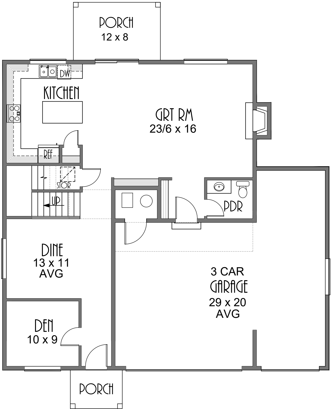
MAIN FLOOR PLAN 1066 SQUARE FEET
