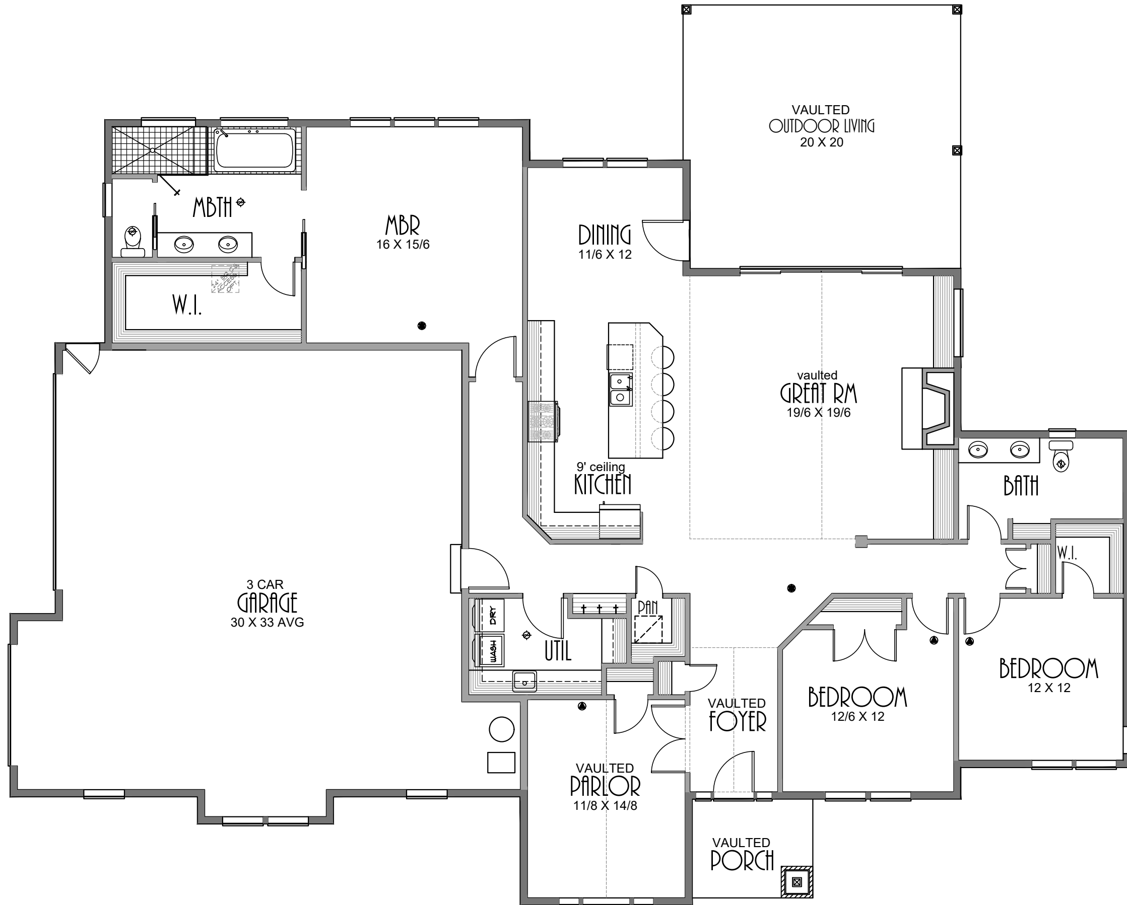
FLOOR PLAN 2395 SQ. FT.
