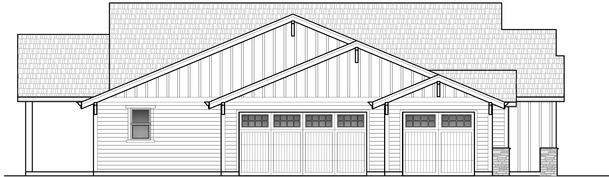
LEFT ELEVATION
