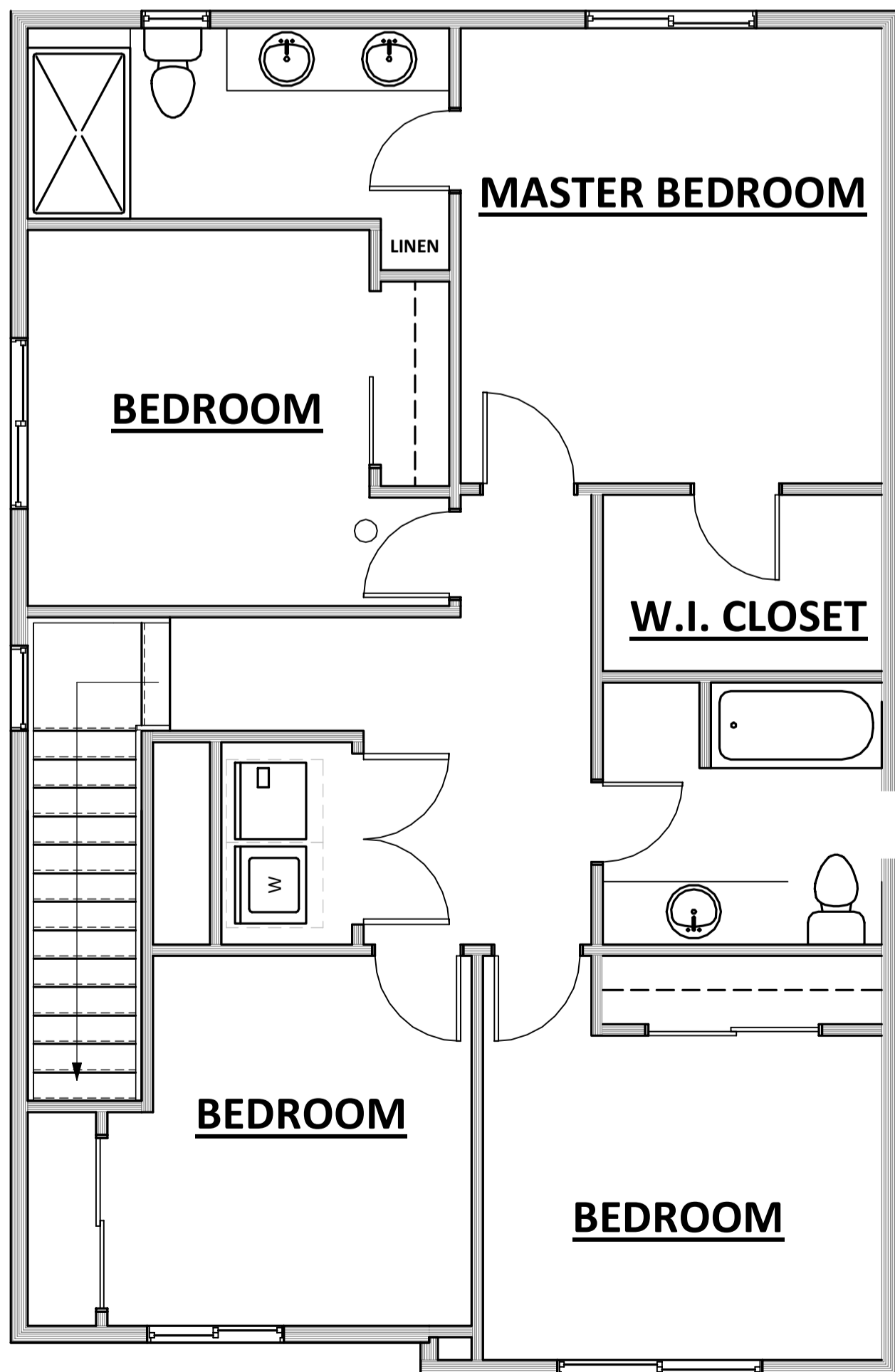
FIRST FLOOR PLAN - 854 S.F.
