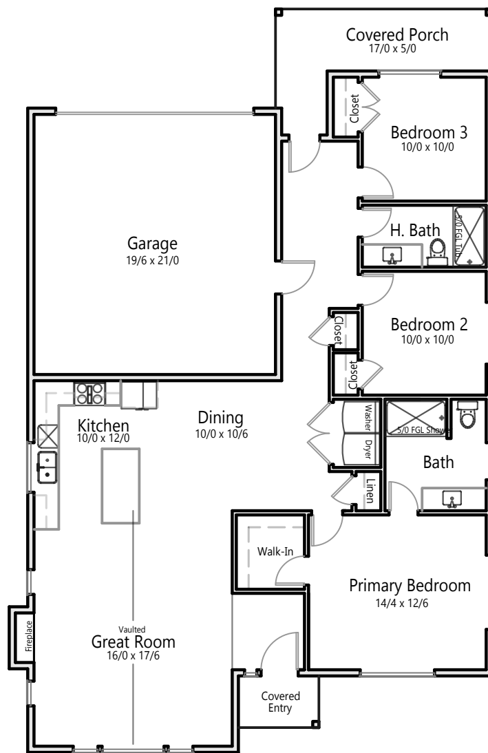
The Laurelwood 1,425 Square Feet
