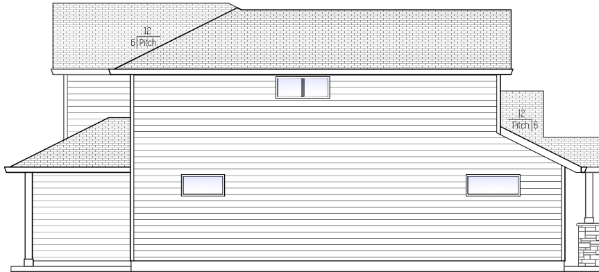
Left Elevation
