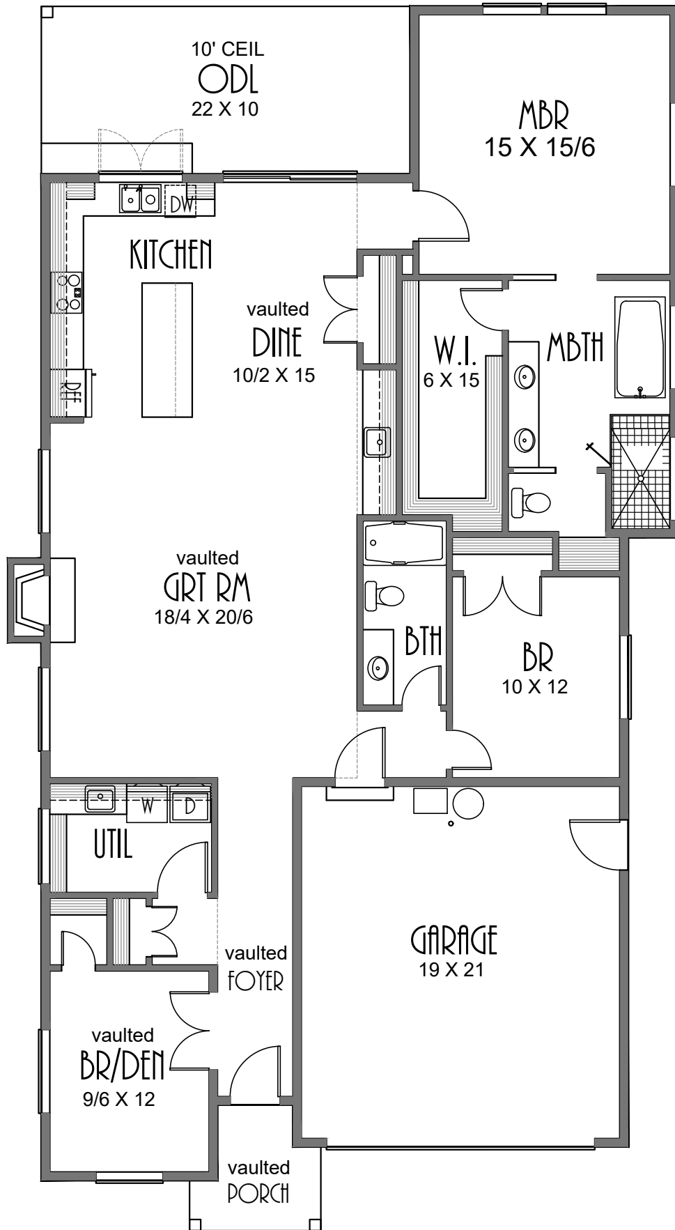
FLOOR PLAN 1825 SQUARE FEET
