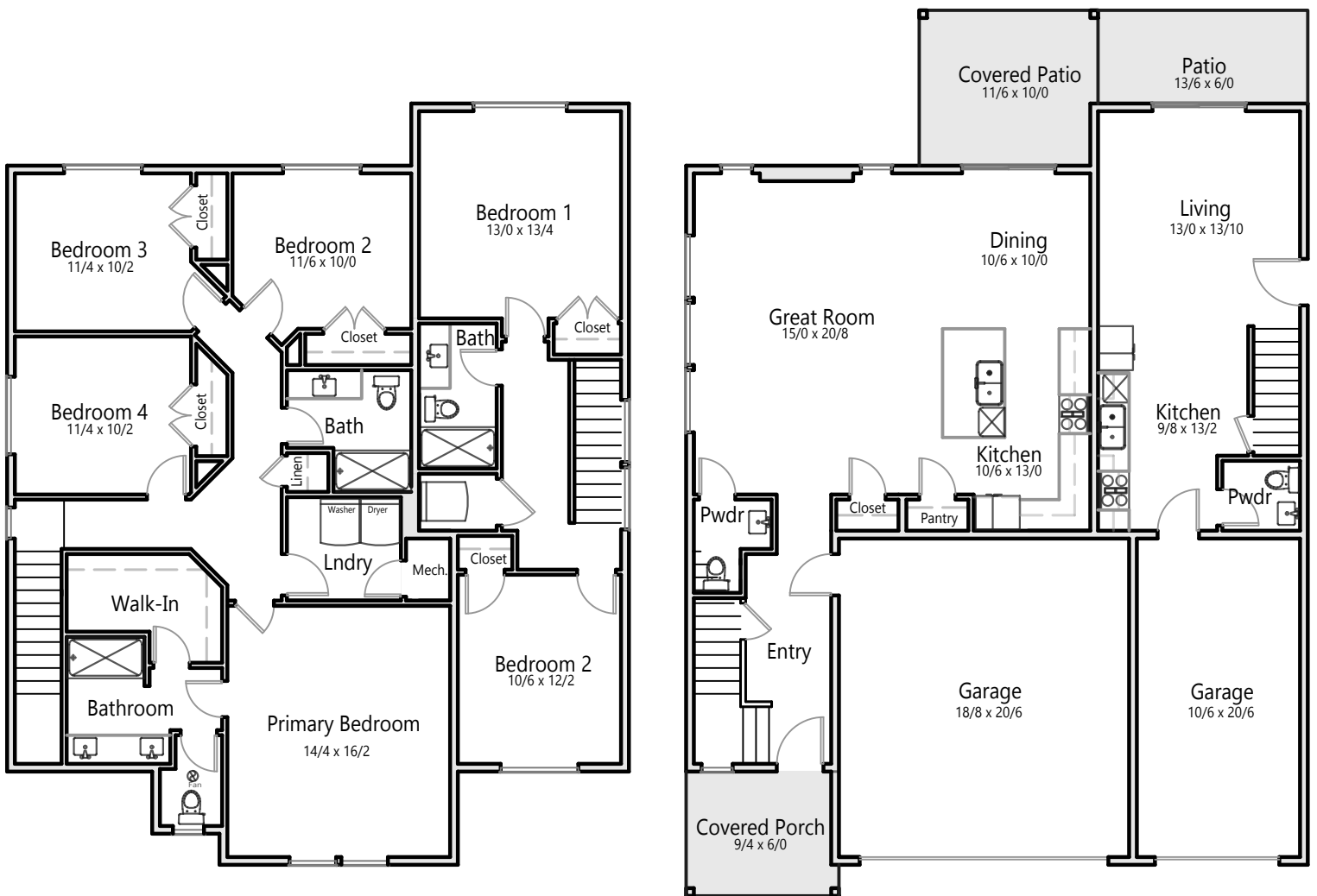
The Oxbow B ADU ADU: 905 Square Feet Main: 1,967 Square Feet
