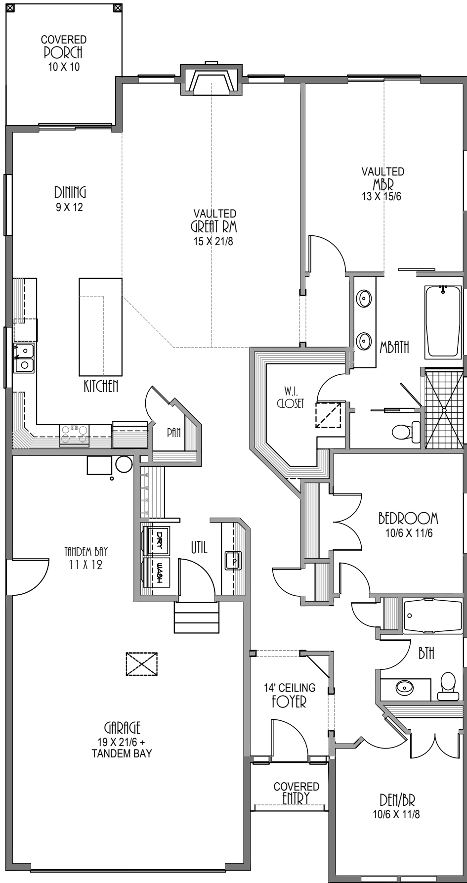
FLOOR PLAN 1828 square feet
