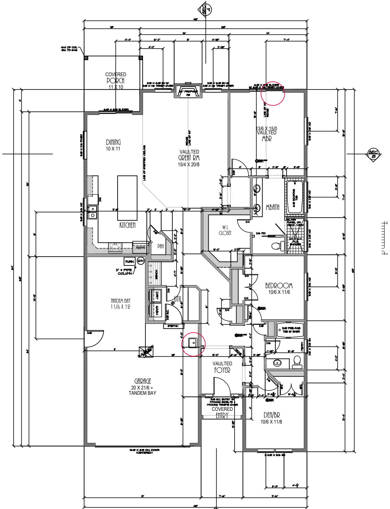
RIPPLEBROOK LOT 22 FLOOR PLAN 1870 square feet
