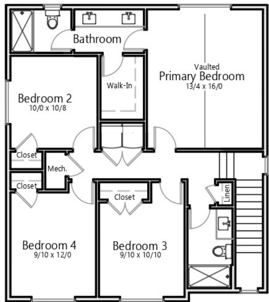
Tygun 3-car 1,684 Square Feet
