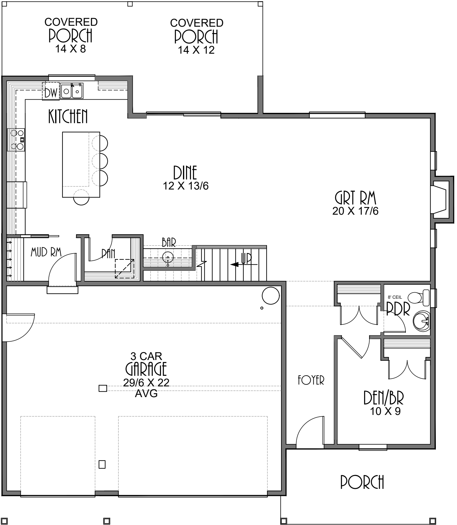
MAIN FLOOR PLAN 1205 SQUARE FEET
